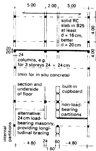
3 Structural system: triple-span beams
